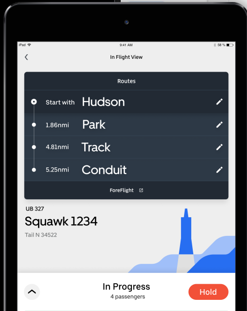
Pilot App
