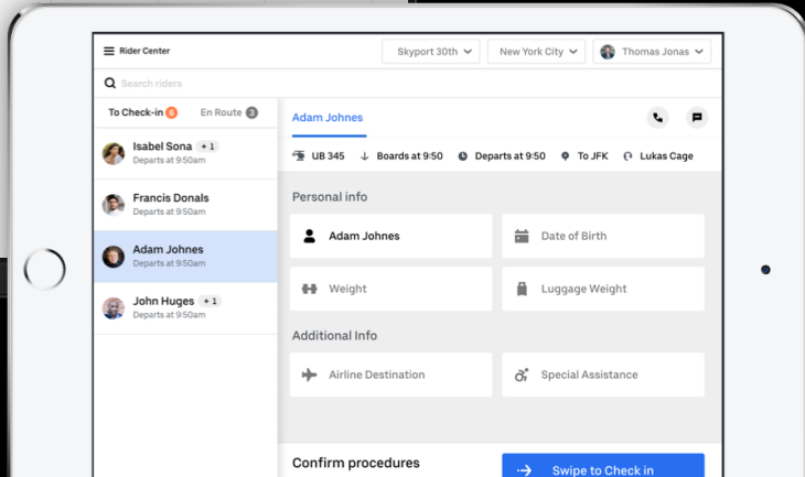
Heliport App
