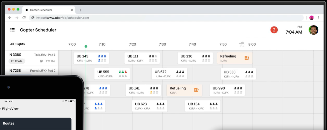
Operations App
