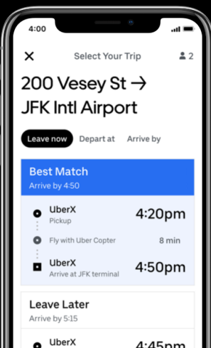
Rider App
